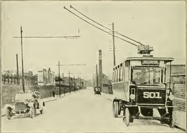
Fig. 17. View Showing How Trackless Trolley Can Draw Up to the Curb
